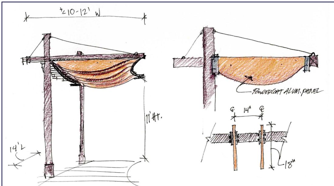
PEACH SHADE SHELTER CONCEPT
