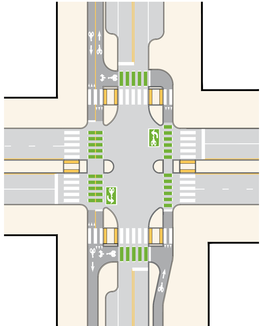
FIGURE 5-37 Two-Way To One-Way Separated Bike Lane Transition
