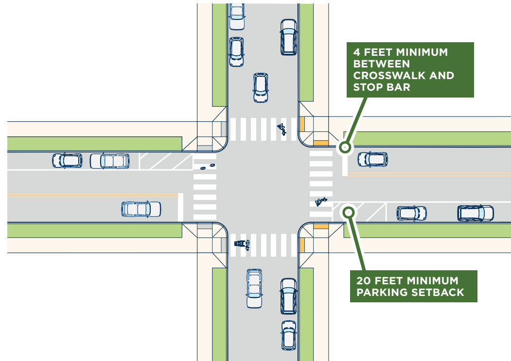
FIGURE 5-20 Crosswalk Placement
