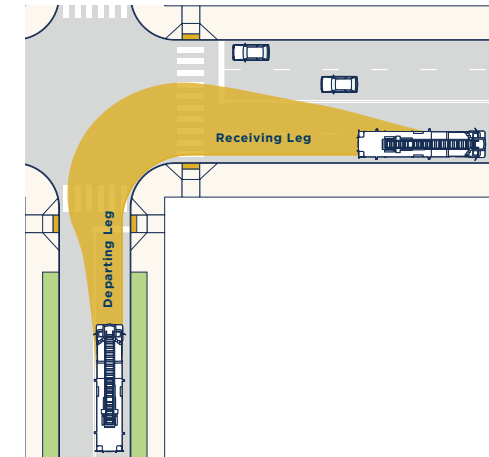
FIGURE 5-6 Degrees of Encroachment
