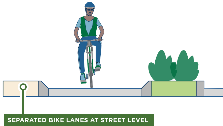
FIGURE 4-15 Separated Bike Lanes at Street Level
