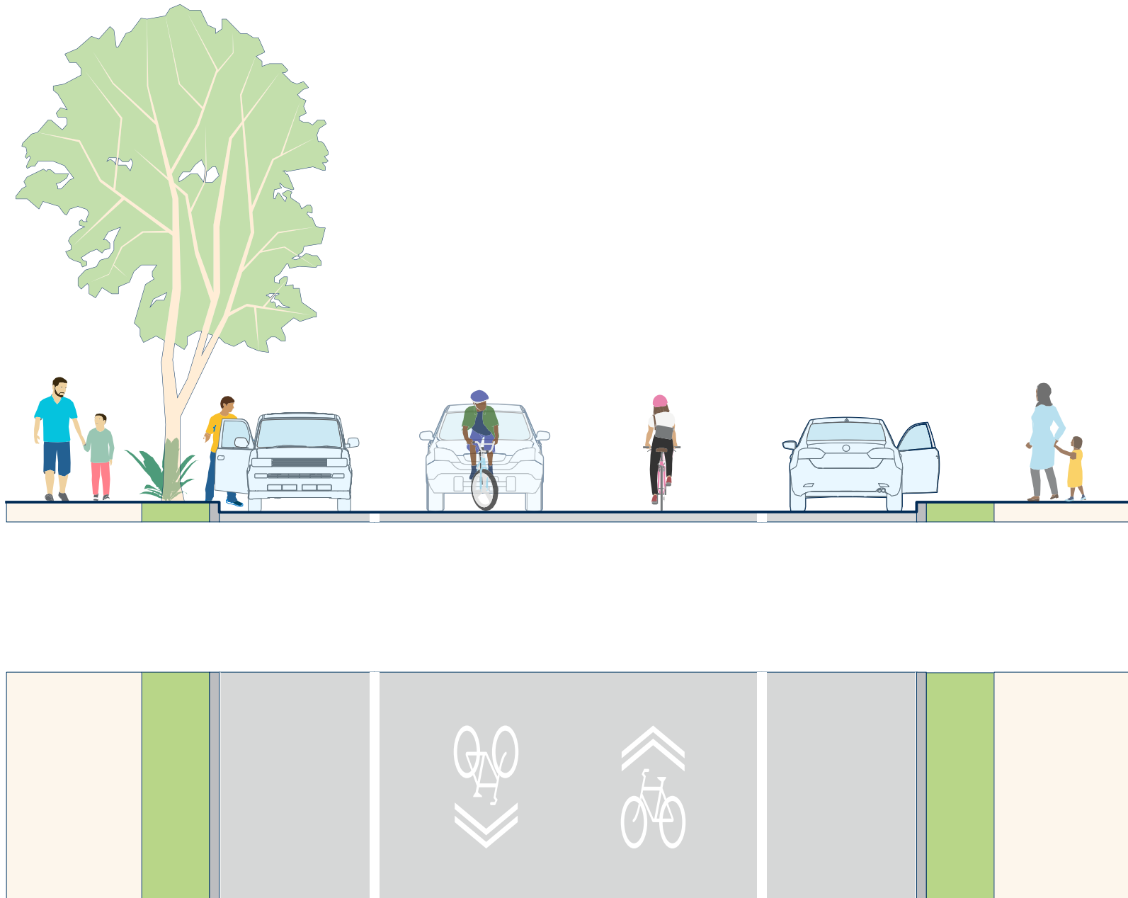
FIGURE 4-20 Neighborhood Bikeway
