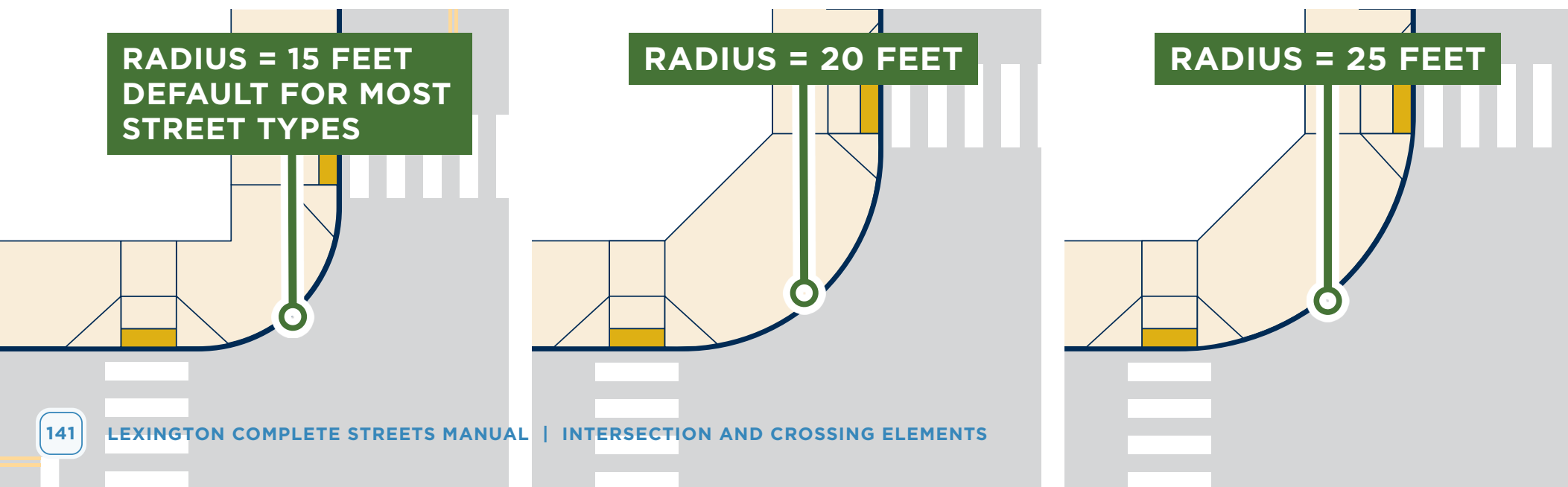
FIGURE 5-3 Common Corner Radius Dimensions
