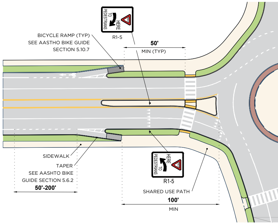
FIGURE 5-40 Bicycle Lane Transition to Shared-Use Path at Roundabout
