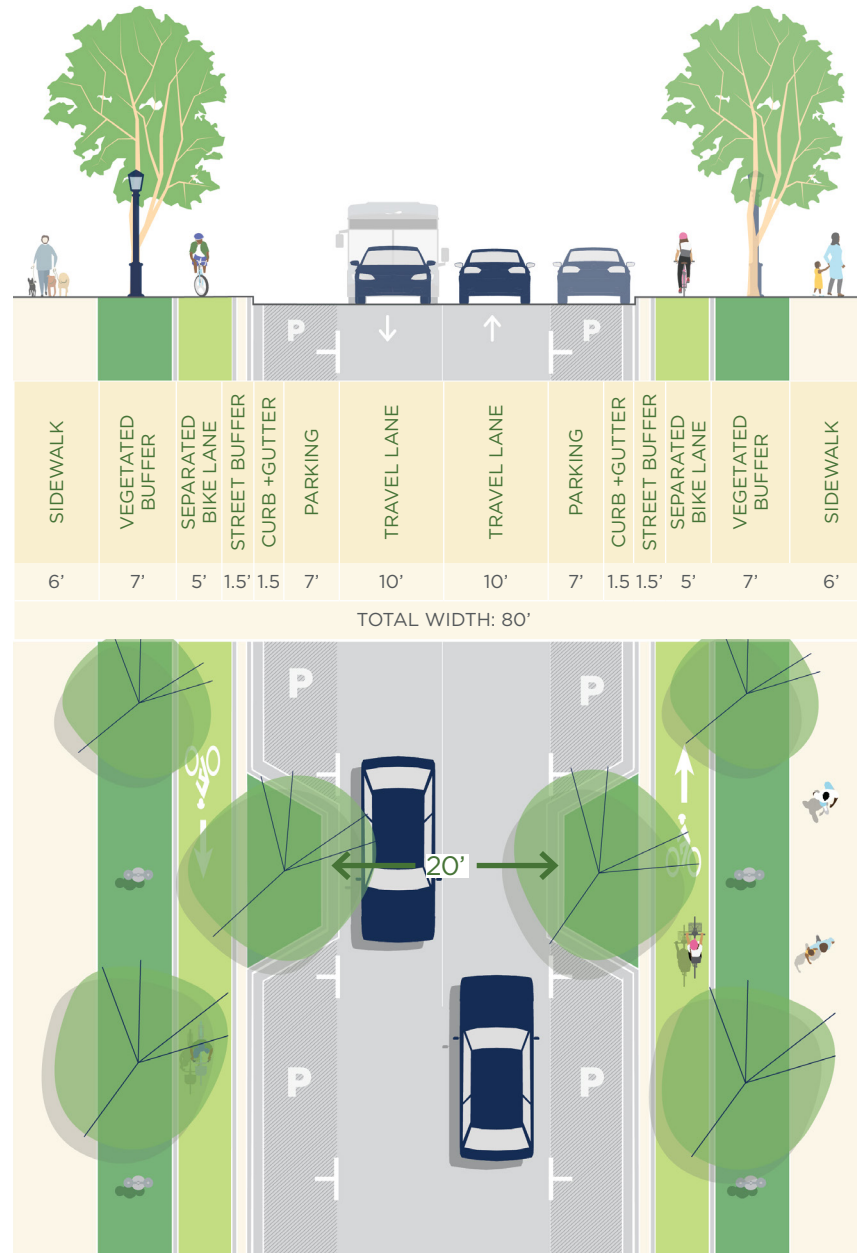
3.1.3.1 LOW TO MODERATE INTENSITY AVENUE (TYPICAL SECTION)
