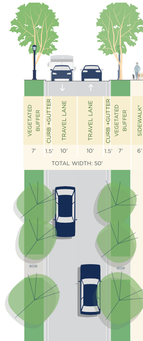
FRONTAGE ROAD (TYPICAL SECTION)
