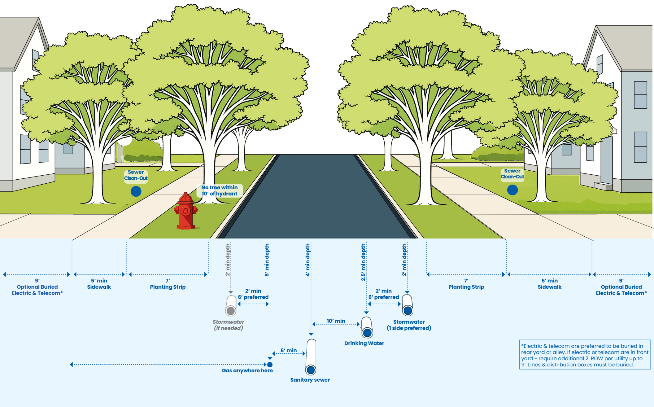
FIGURE 4-43 Utility Placement for New Developments
