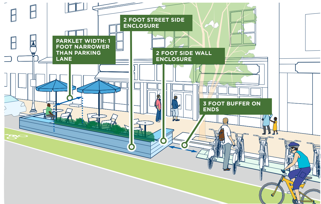
FIGURE 4-30 Parklets
