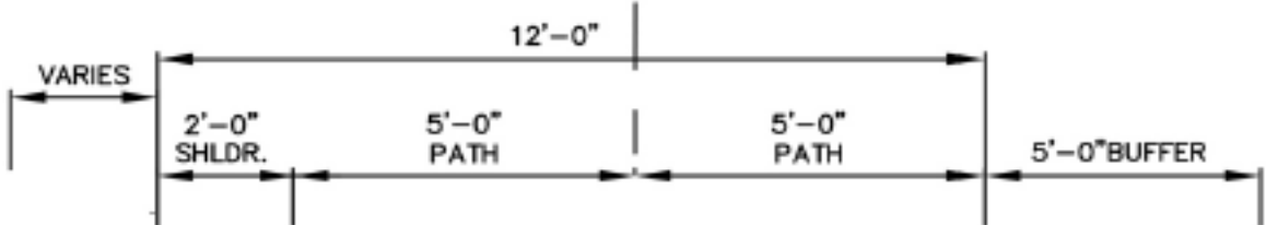
Retaining Walls on Highbank Side
